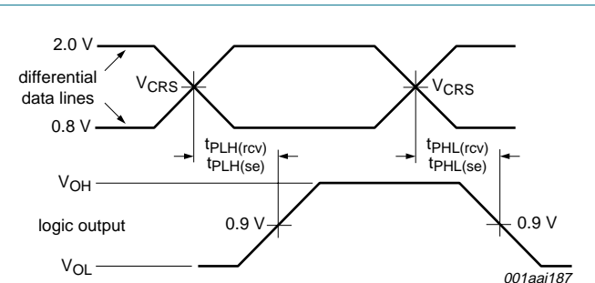
Fig 29. Timing of DP and DM to RX_RCV, RX_DP and RX_DM
