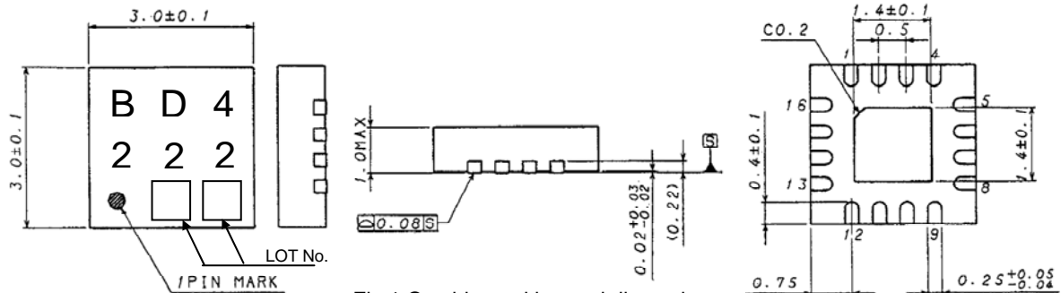
Fig.1 Outside marking and dimension
