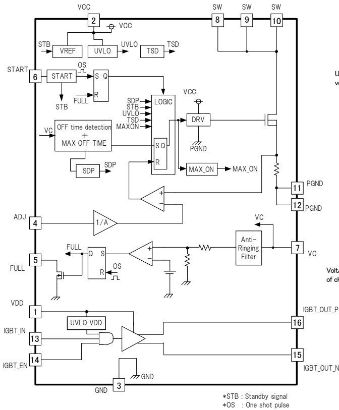
Fig.3 Block diagram
