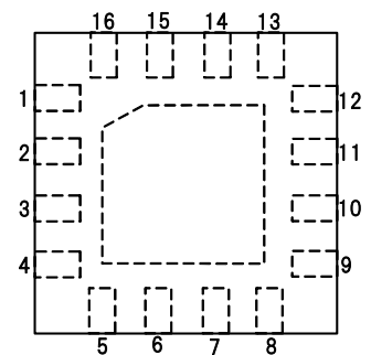
Fig.3 TOP VIEW
