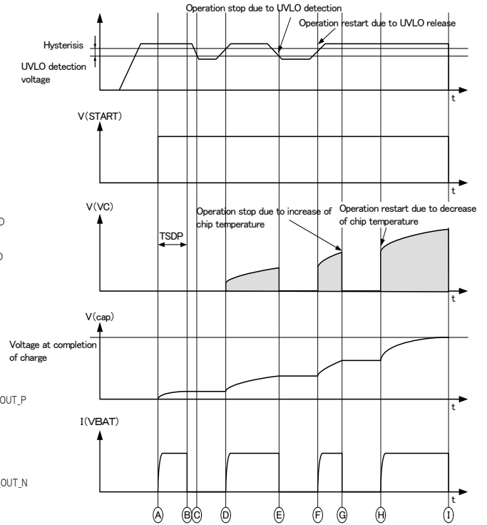
Fig.4 Timing Chart: Under Protective Circuit Operation
