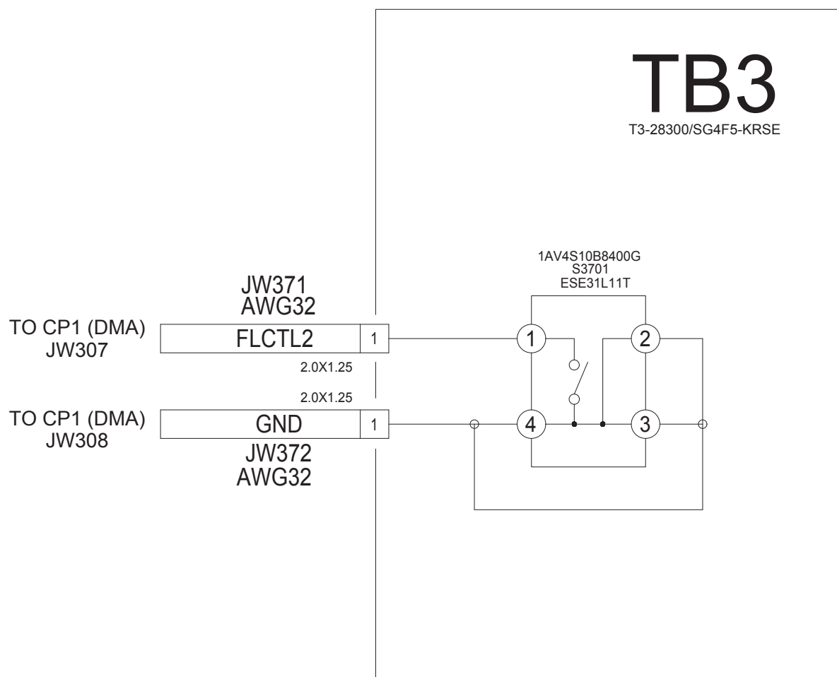
MODEL: EC-WB5500 CIRCUIT DIAGRAM: TB3
