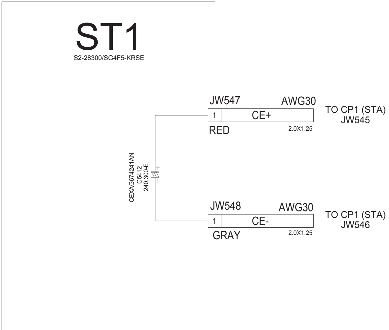
MODEL: EC-WB5500 CIRCUIT DIAGRAM: ST1
