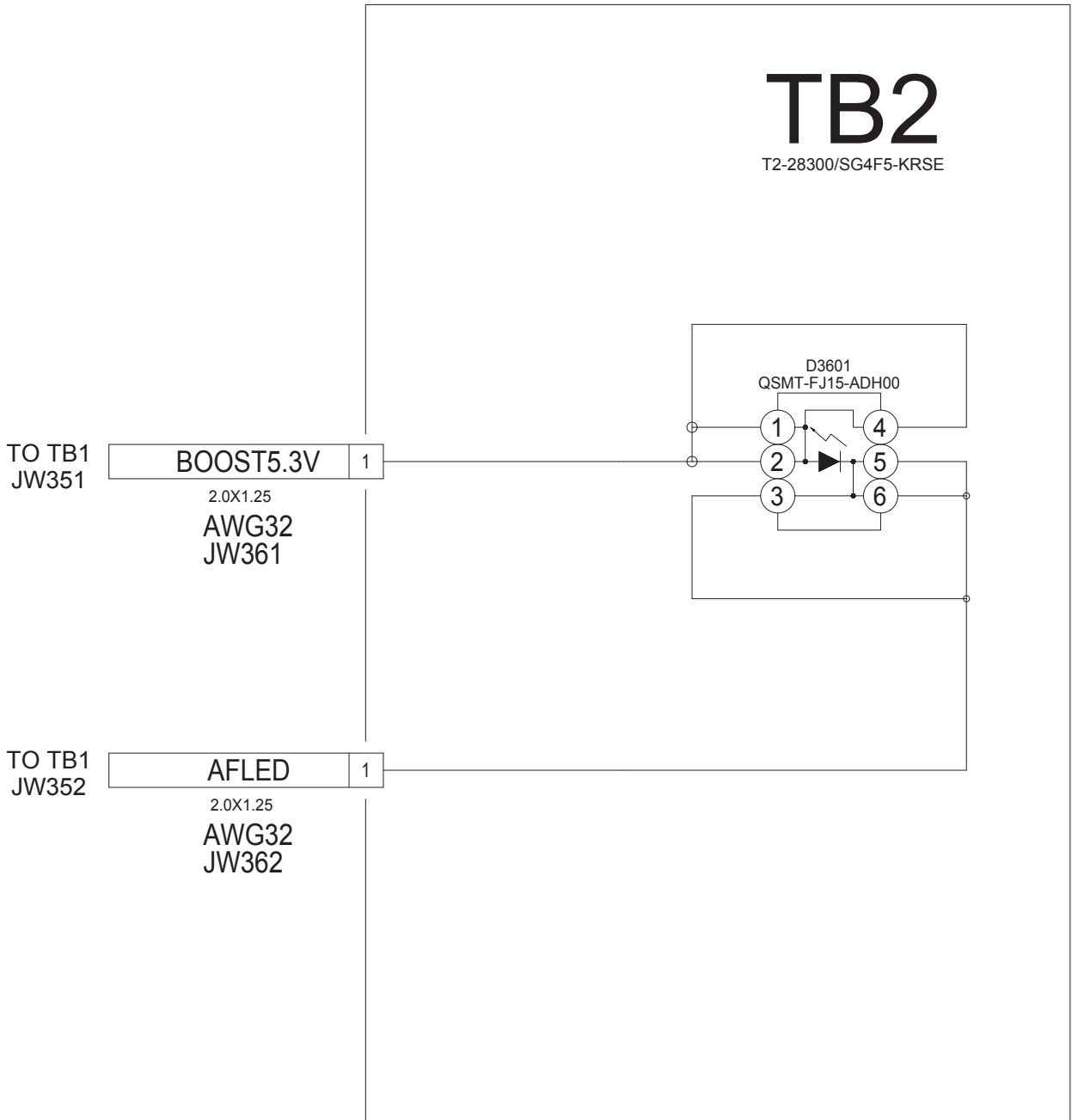
MODEL: EC-WB5500 CIRCUIT DIAGRAM: TB2
