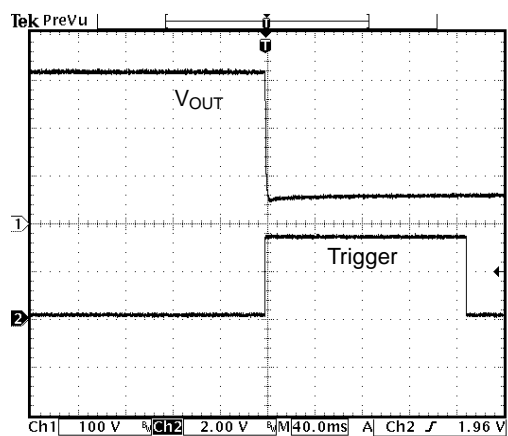
Fig. 4 Trigger waveform
