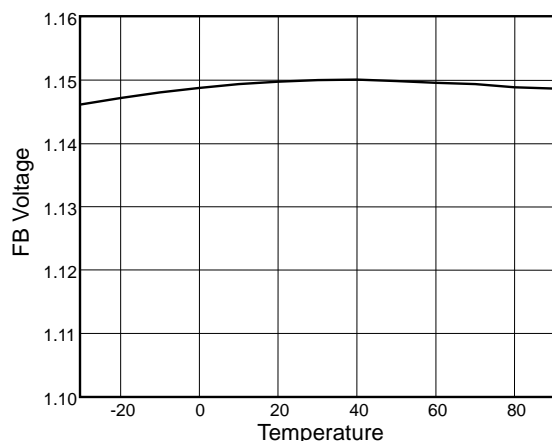
Fig. 6 FB Voltage vs. Temperature
