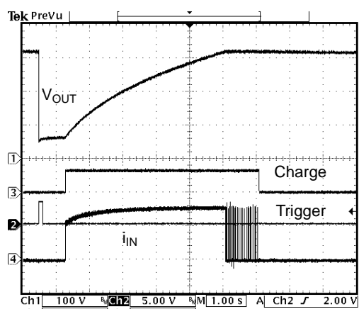
Fig. 5 Recharging waveform V_{IN}=3.0V
