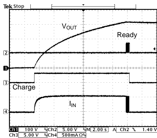
Fig. 3 Charging waveform V_{IN}=2.0V
